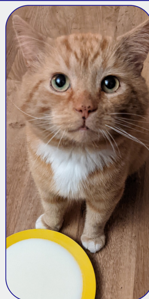
Cats
